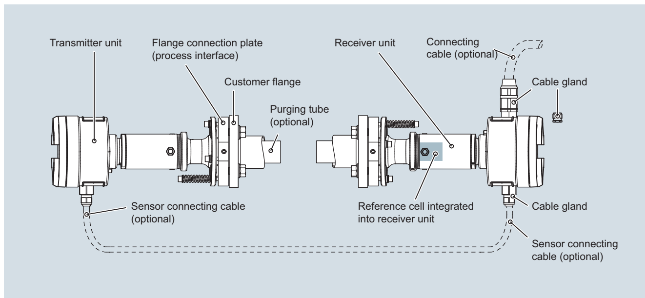
Design of the non-Ex version of the SITRANS SL system
